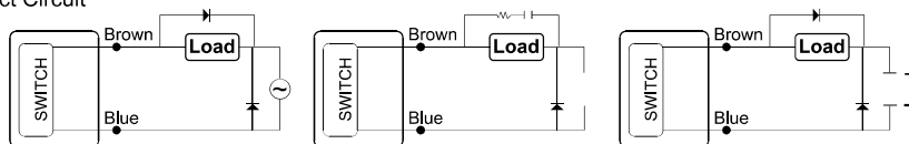
External Protect Circuit
