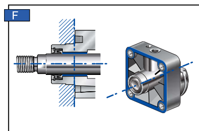
Machined to get centering and surface finishing.
